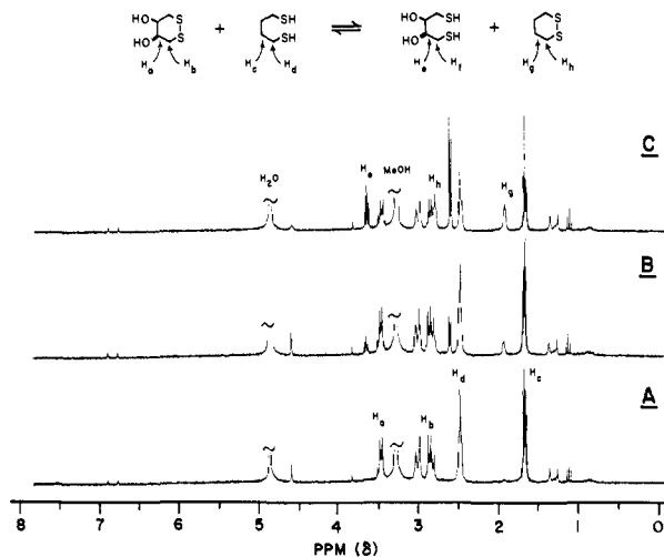
Figure 7. Reaction of \text{DTT}^{\text{ox}} with 1,4-butanedithiol as monitored by ^1\text{H} NMR. Solution is initially 1 mM \text{DTT}^{\text{ox}} and 1 mM 1,4-butanedithiol in 1:1 methanol- d_4 /aqueous buffer (0.1 M phosphate, pH 7). Spectra shown correspond to an equilibration: (A) at the start of the experiment; (B) during the equilibration; (C) at final equilibrium.
